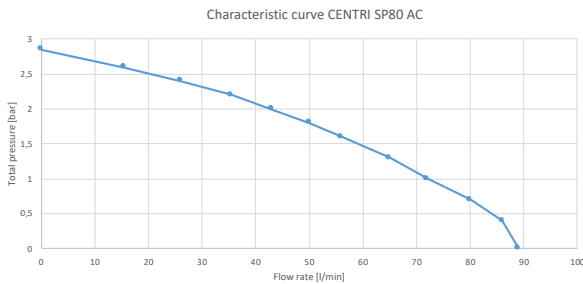
dispensing volume submersible pump CENTRI SP80
